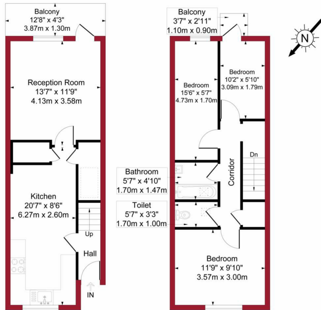
First Floor Gross Internal Floor Area 394 sq ft / 36.6 sq m
