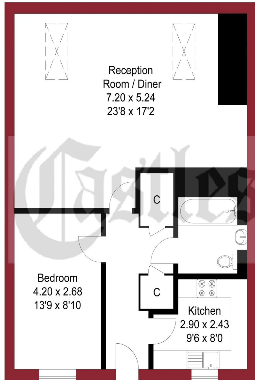
FOURTH FLOOR
